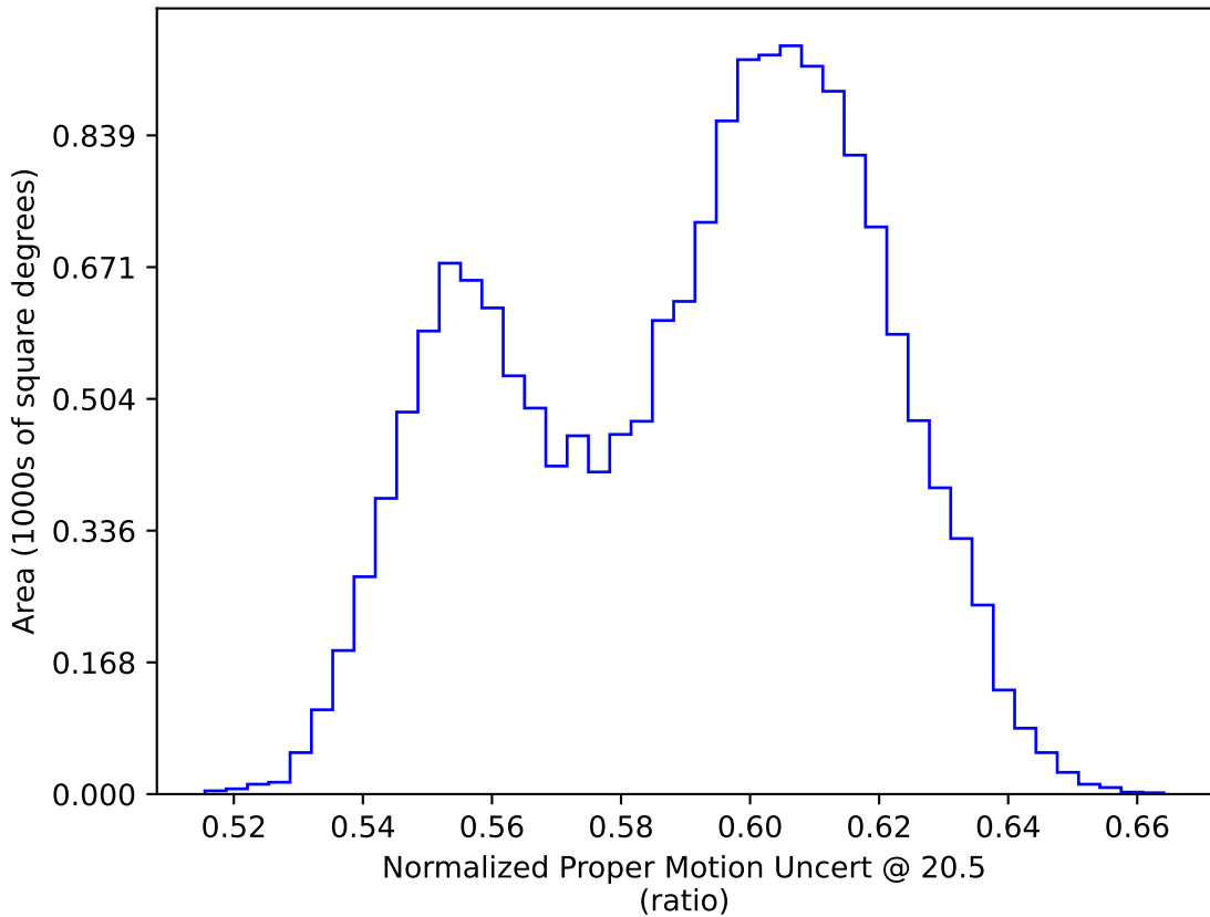
mw_roll_bulge_v3.3_10yrs WFD: Normalized Proper Motion Uncert @ 20.5
