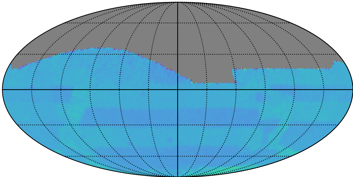
mw_roll_bulge_v3.3_10yrs All sky: Normalized Proper Motion Uncert @ 20.5
