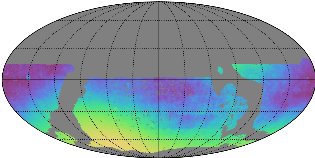
mw_roll_bulge_v3.3_10yrs WFD: Normalized Parallax Uncert @ 24.0
