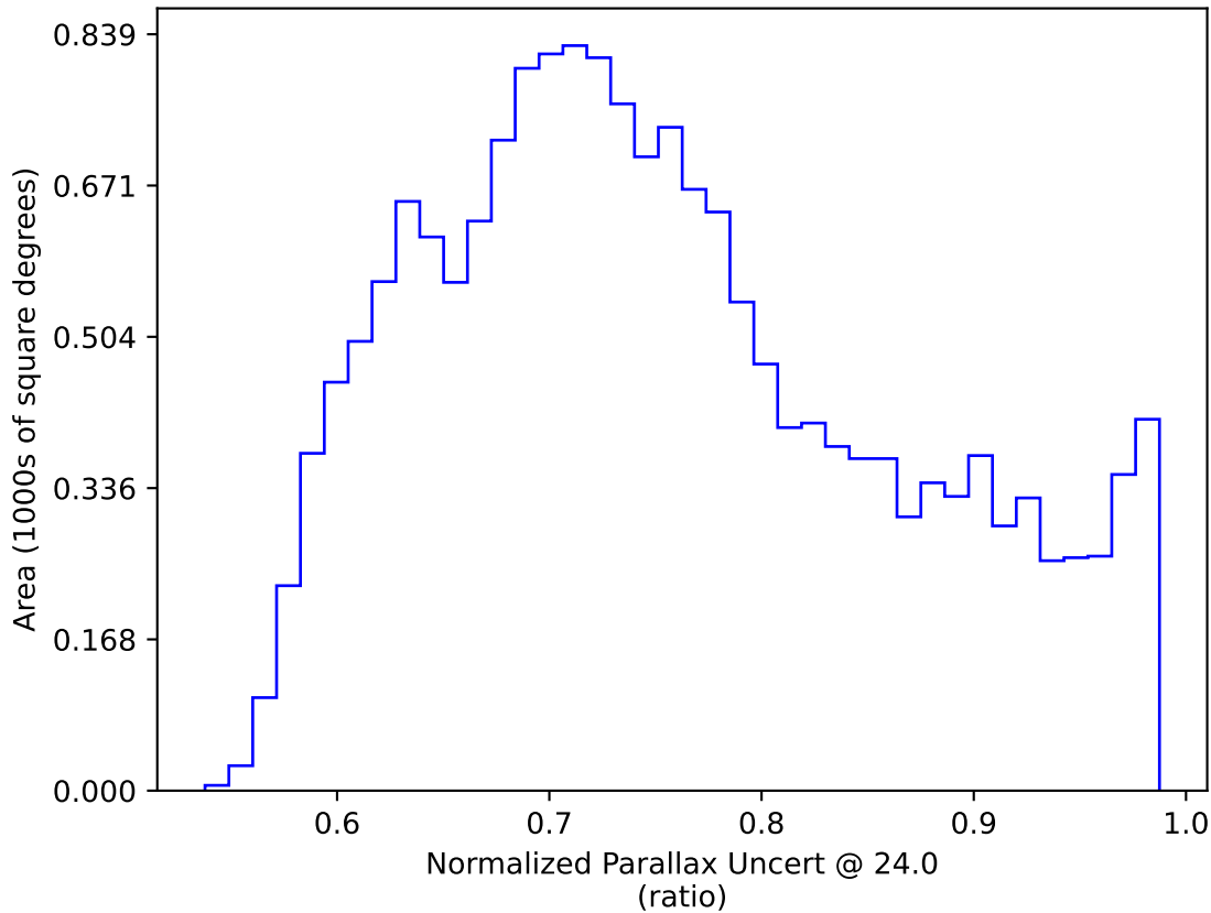
mw_roll_bulge_v3.3_10yrs WFD: Normalized Parallax Uncert @ 24.0
