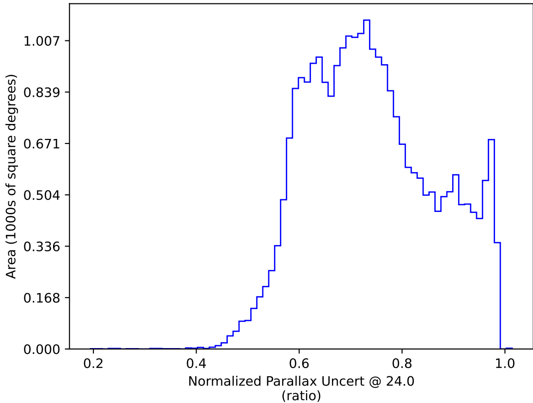
mw_roll_bulge_v3.3_10yrs All sky: Normalized Parallax Uncert @ 24.0
