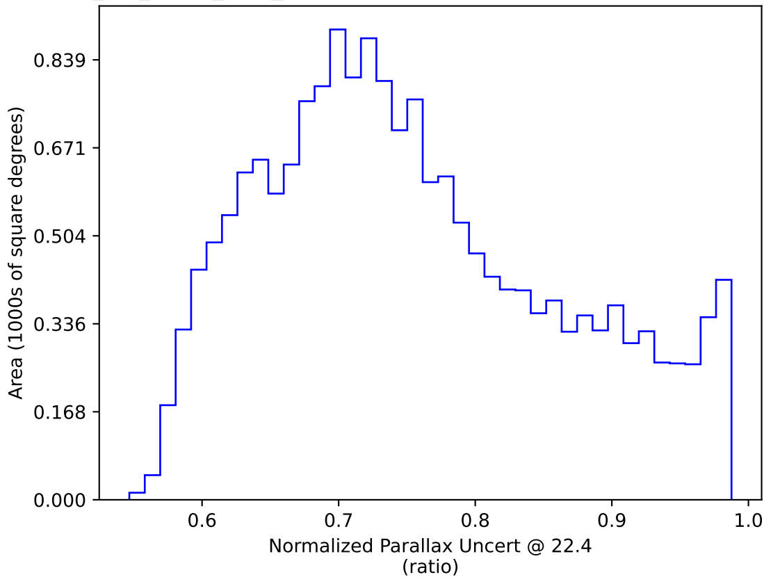
mw_roll_bulge_v3.3_10yrs WFD: Normalized Parallax Uncert @ 22.4
