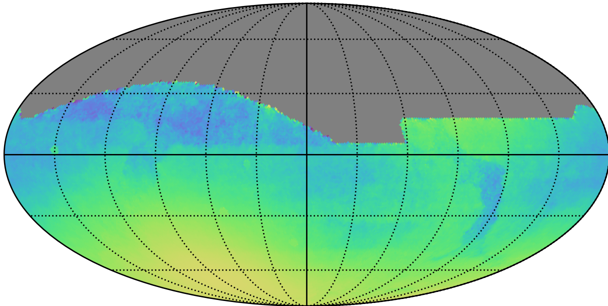
mw_roll_bulge_v3.3_10yrs All sky: Normalized Parallax Uncert @ 22.4
