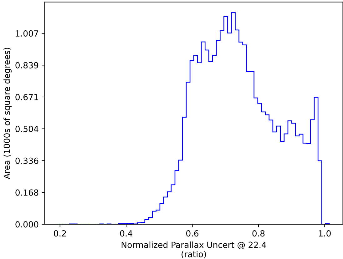
mw_roll_bulge_v3.3_10yrs All sky: Normalized Parallax Uncert @ 22.4
