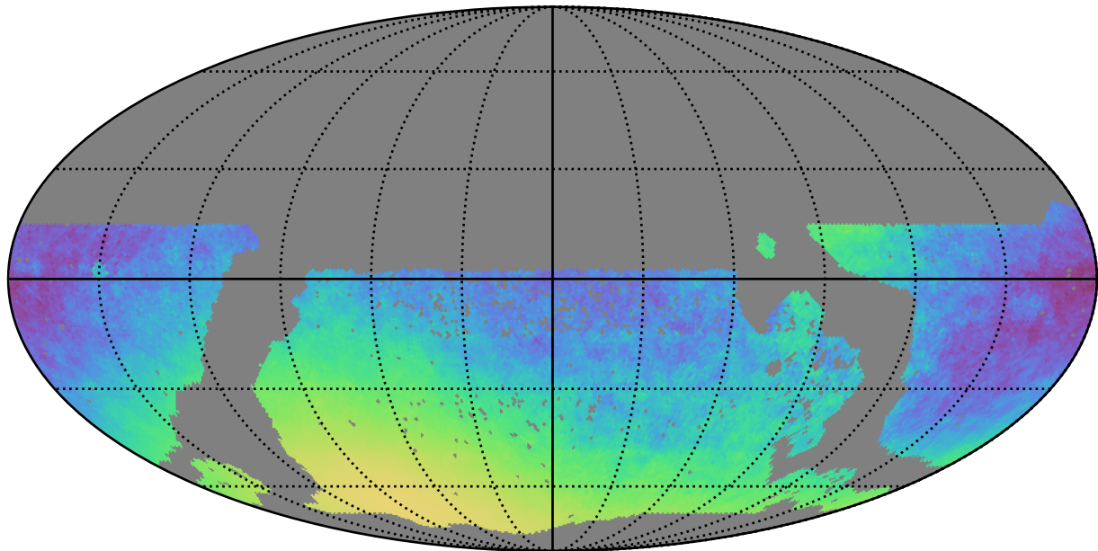
mw_roll_bulge_v3.3_10yrs WFD y band only: Normalized Parallax Uncert @ 21.3
