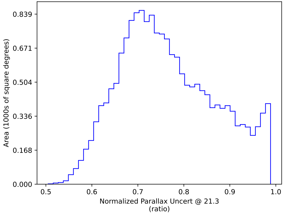
mw_roll_bulge_v3.3_10yrs WFD y band only: Normalized Parallax Uncert @ 21.3
