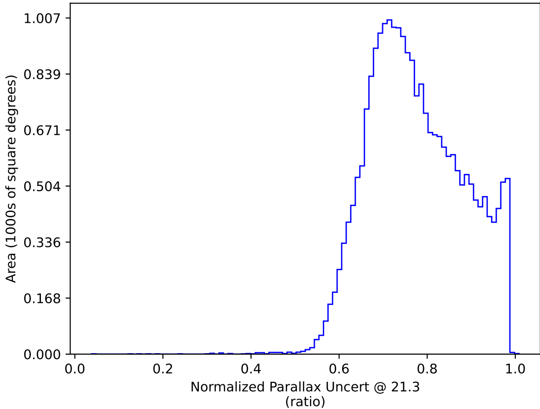
mw_roll_bulge_v3.3_10yrs All sky y band only: Normalized Parallax Uncert @ 21.3
