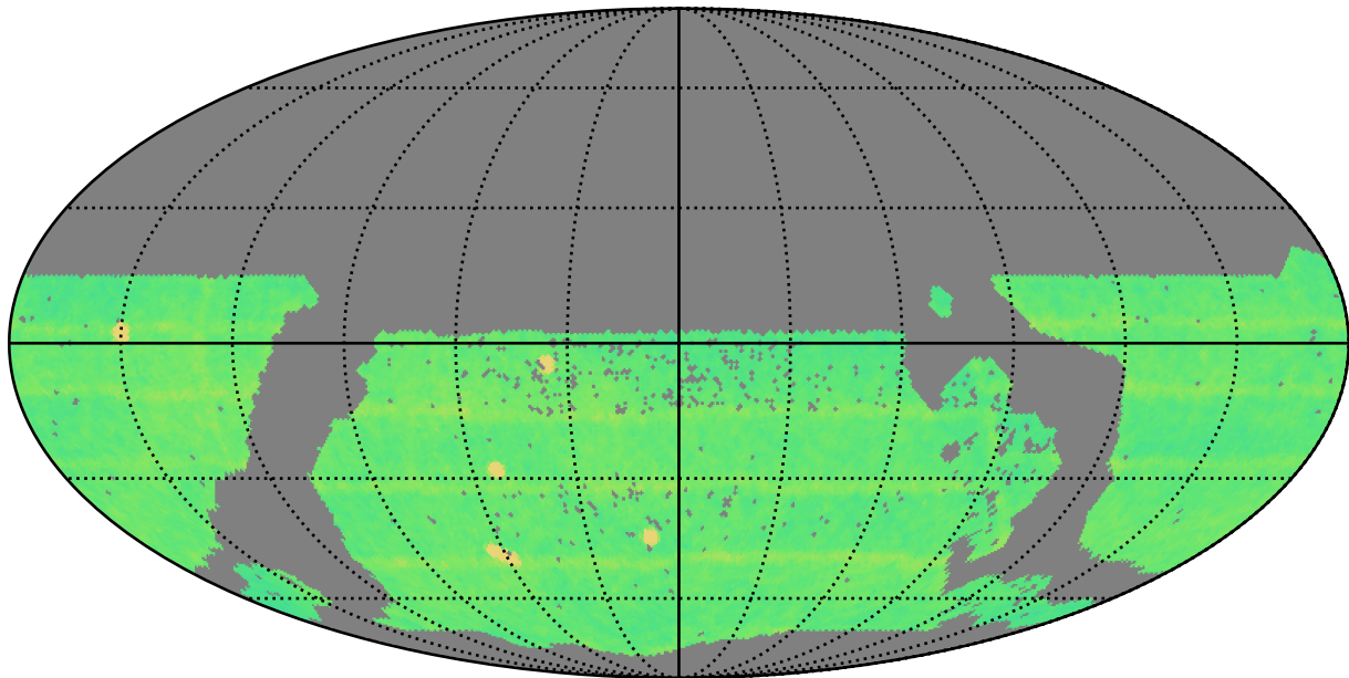
mw_roll_bulge_v3.3_10yrs WFD all bands: N Unique Nights
