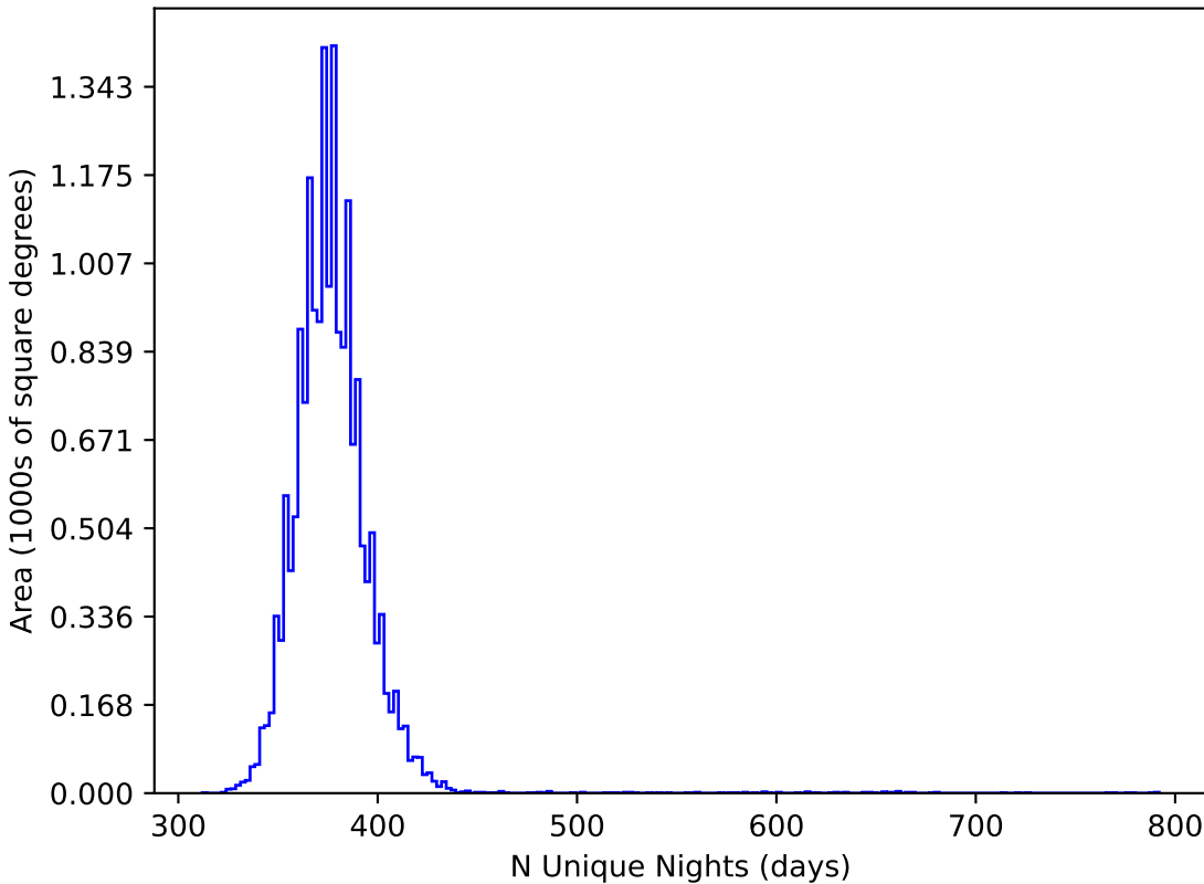
mw_roll_bulge_v3.3_10yrs WFD all bands: N Unique Nights
