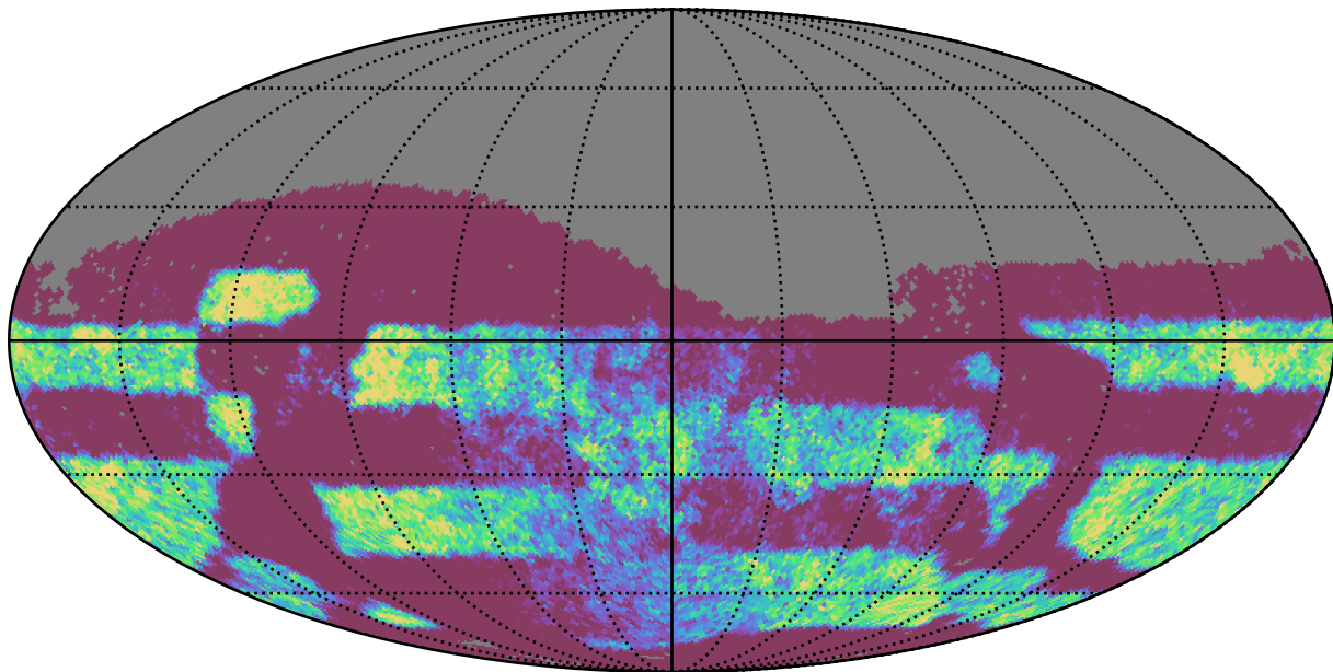
mw_roll_bulge_v3.3_10yrs Yr 3-4 z band: NVisits
