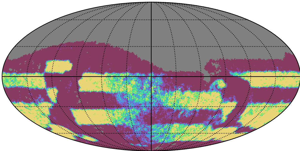
mw_roll_bulge_v3.3_10yrs Yr 3-4 r band: NVisits
