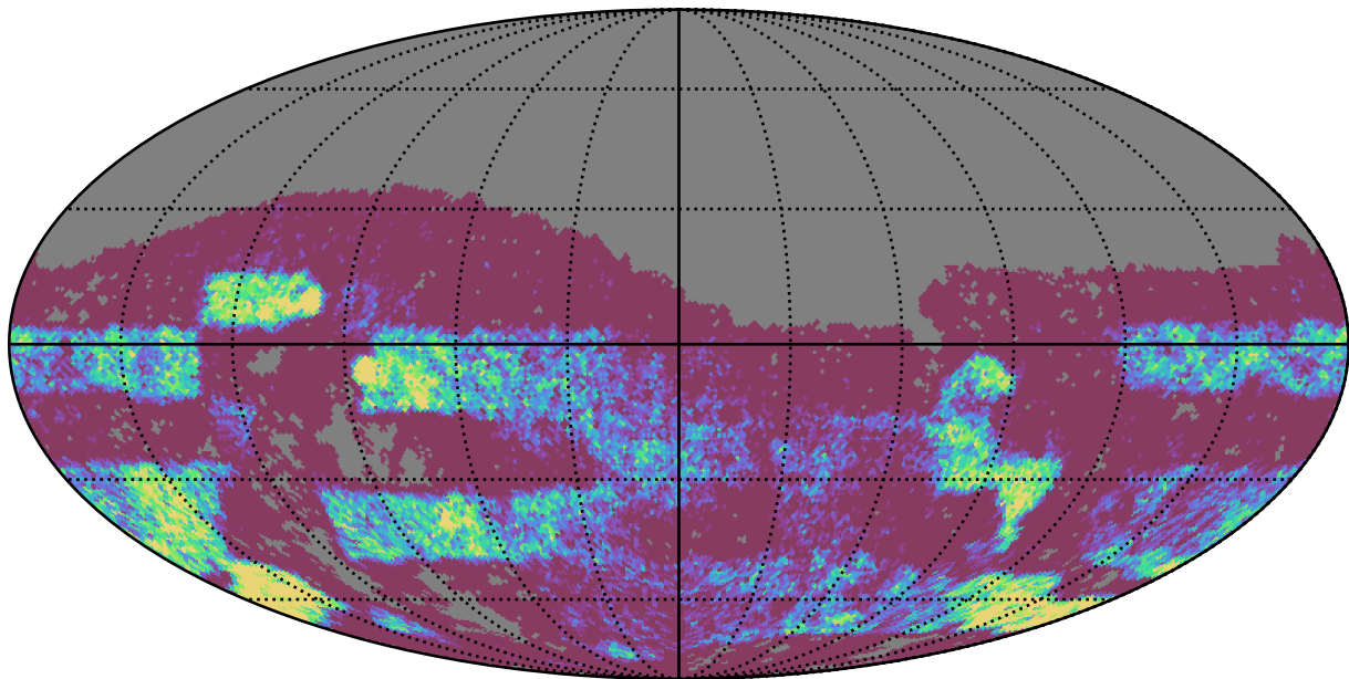
mw_roll_bulge_v3.3_10yrs Yr 3-4 g band: NVisits
