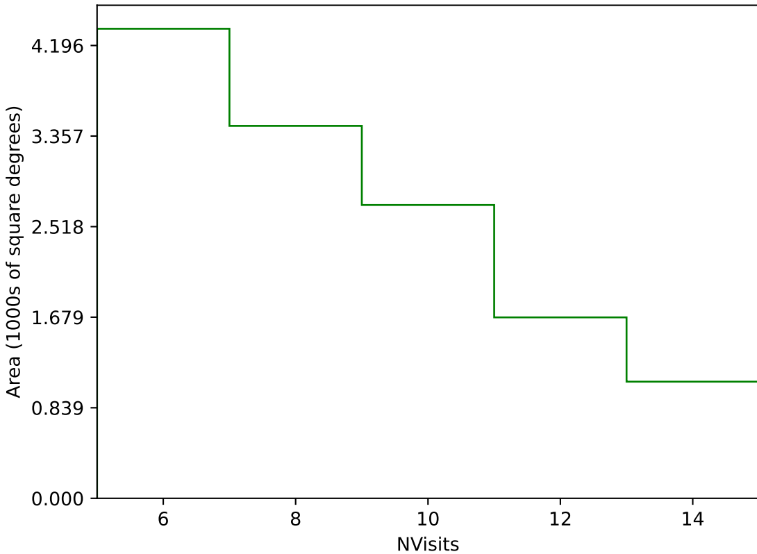
mw_roll_bulge_v3.3_10yrs Yr 3-4 g band: NVisits
