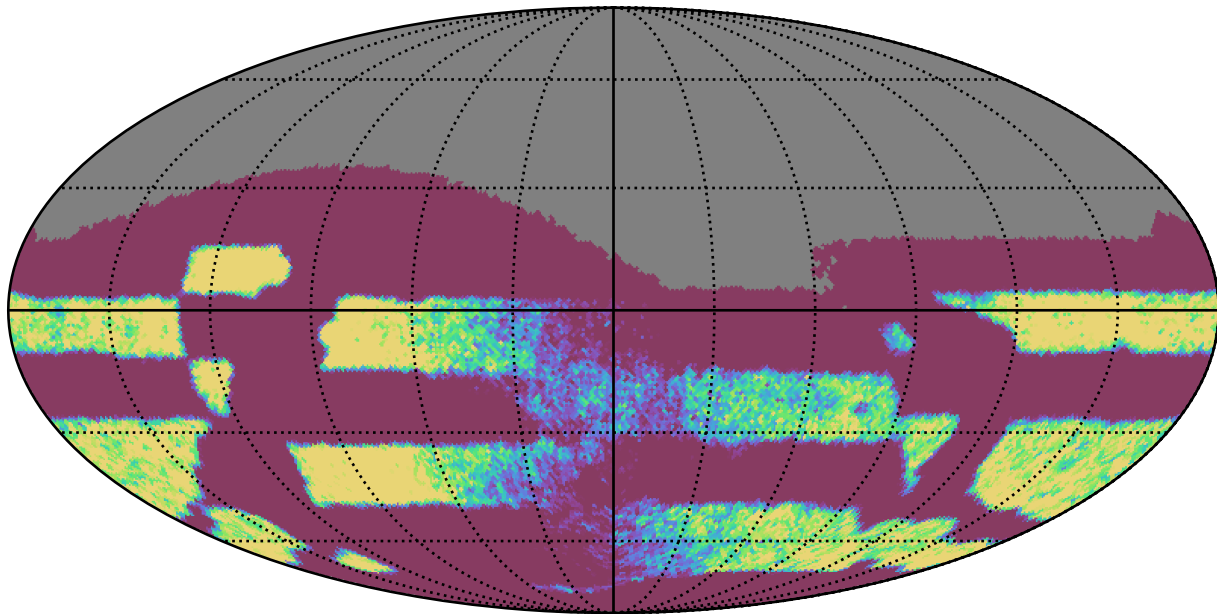
mw_roll_bulge_v3.3_10yrs Yr 3-4 all bands: NVisits
