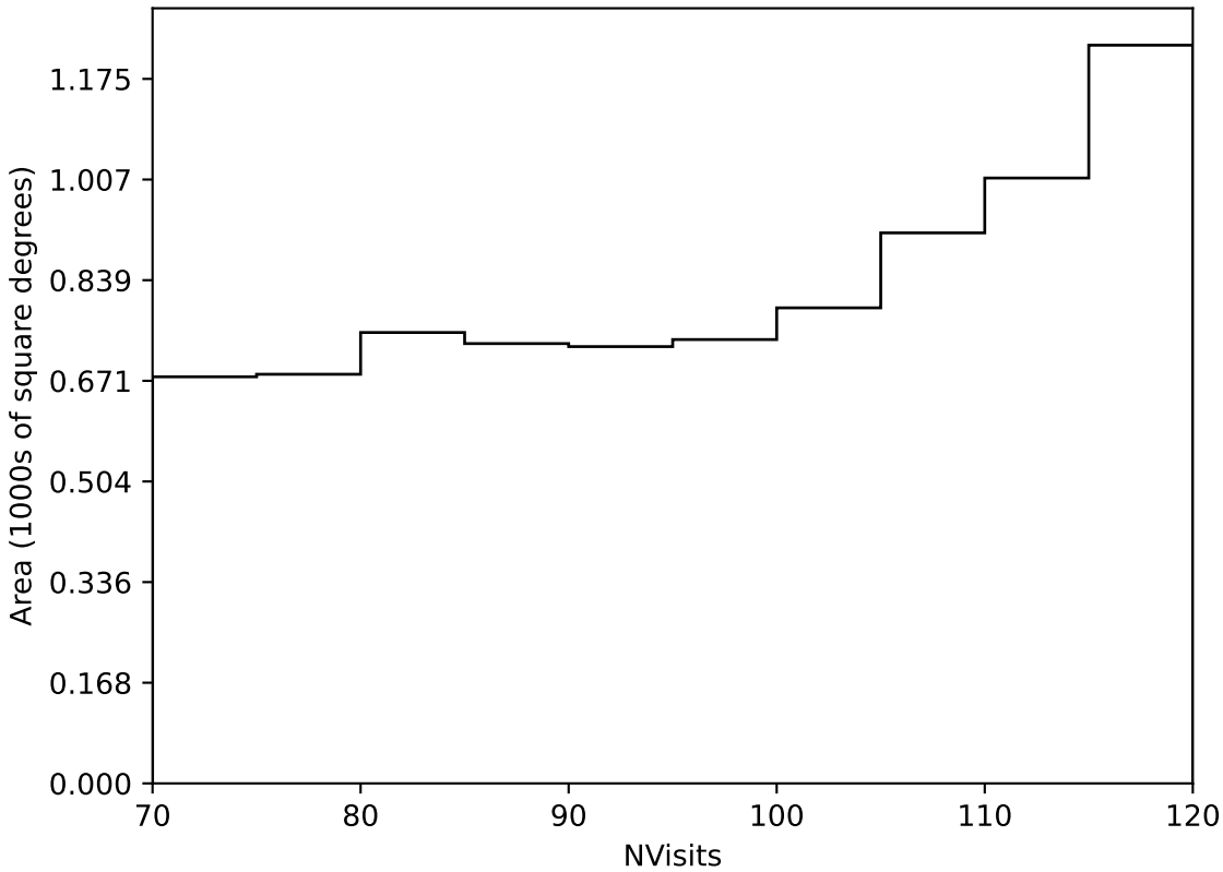
mw_roll_bulge_v3.3_10yrs Yr 3-4 all bands: NVisits
