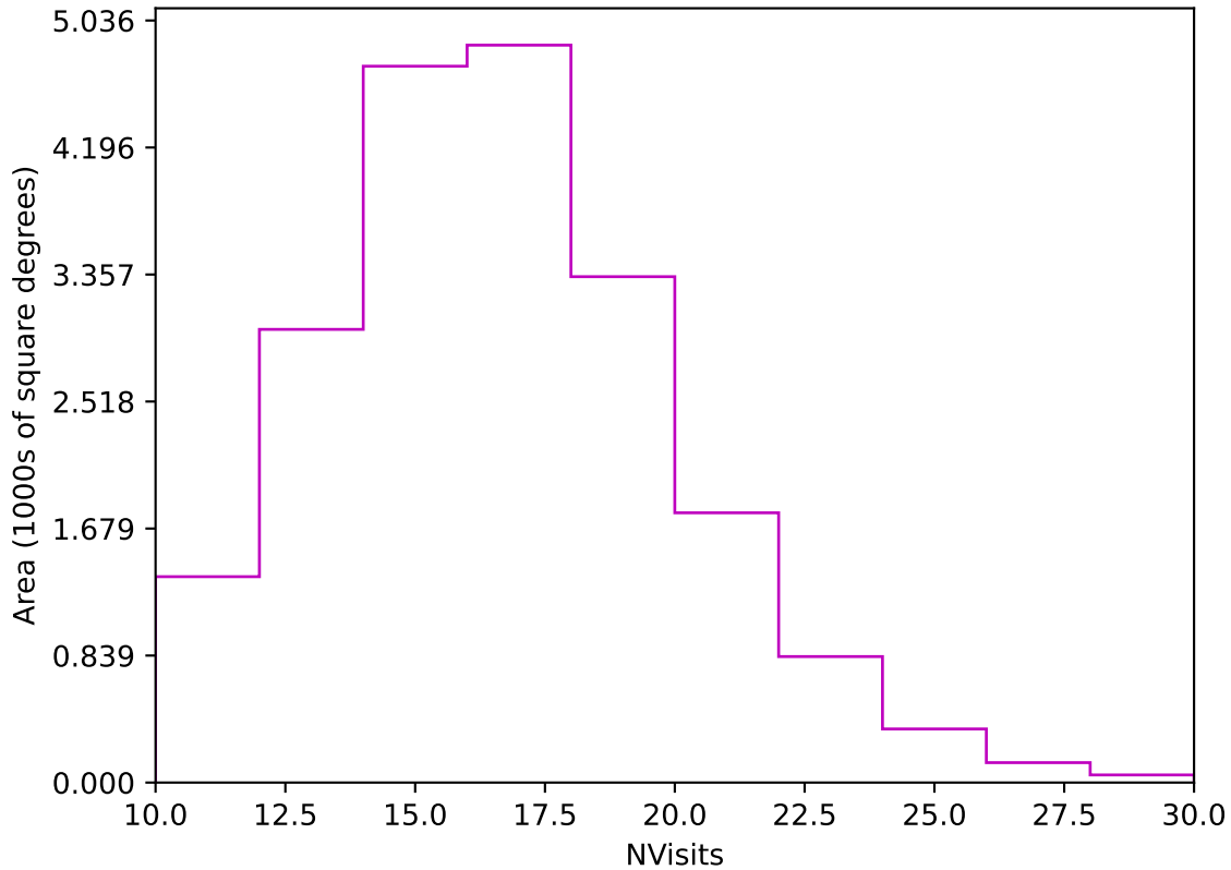
mw_roll_bulge_v3.3_10yrs Yr 1 z band: NVisits
