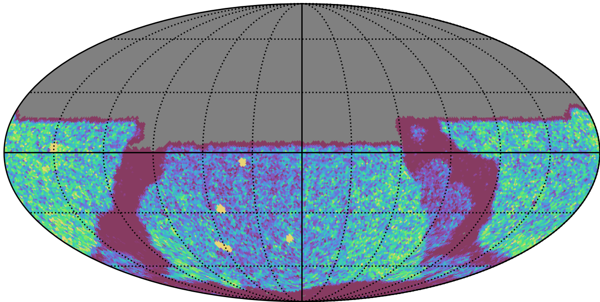
mw_roll_bulge_v3.3_10yrs Yr 1 y band: NVisits
