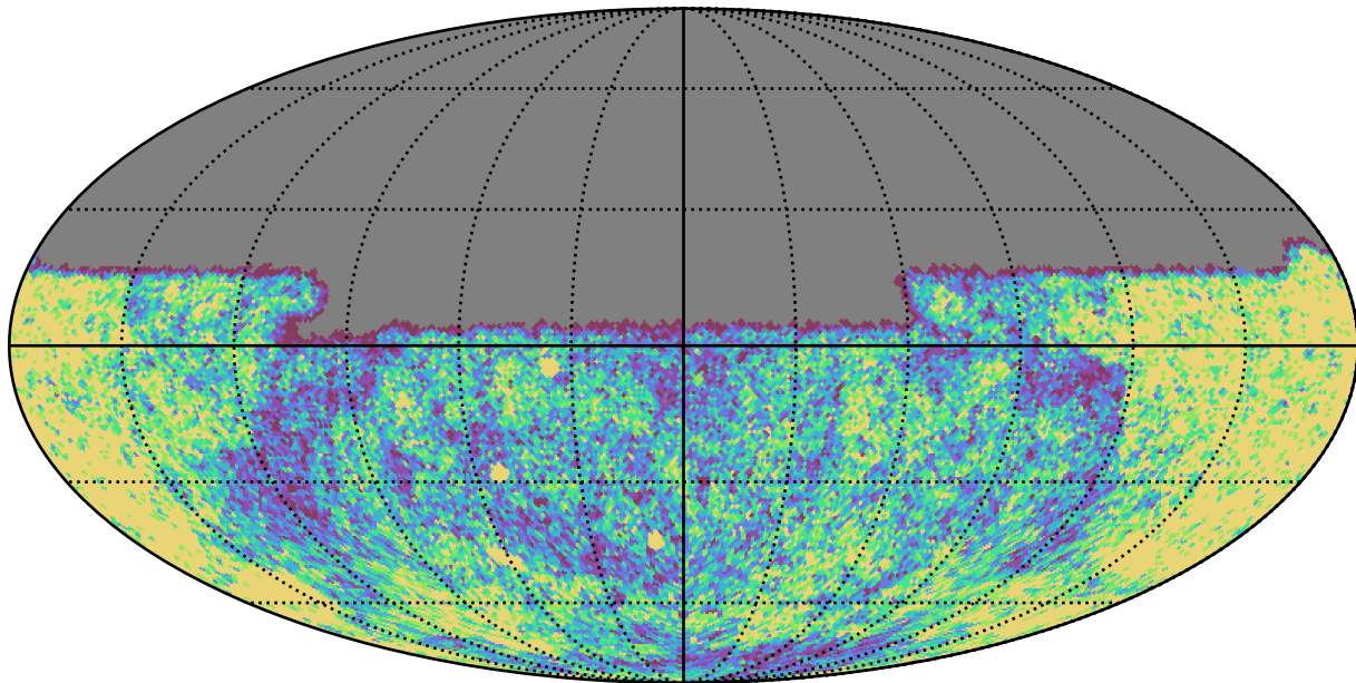
mw_roll_bulge_v3.3_10yrs Yr 1 u band: NVisits
