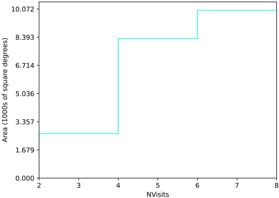
mw_roll_bulge_v3.3_10yrs Yr 1 u band: NVisits
