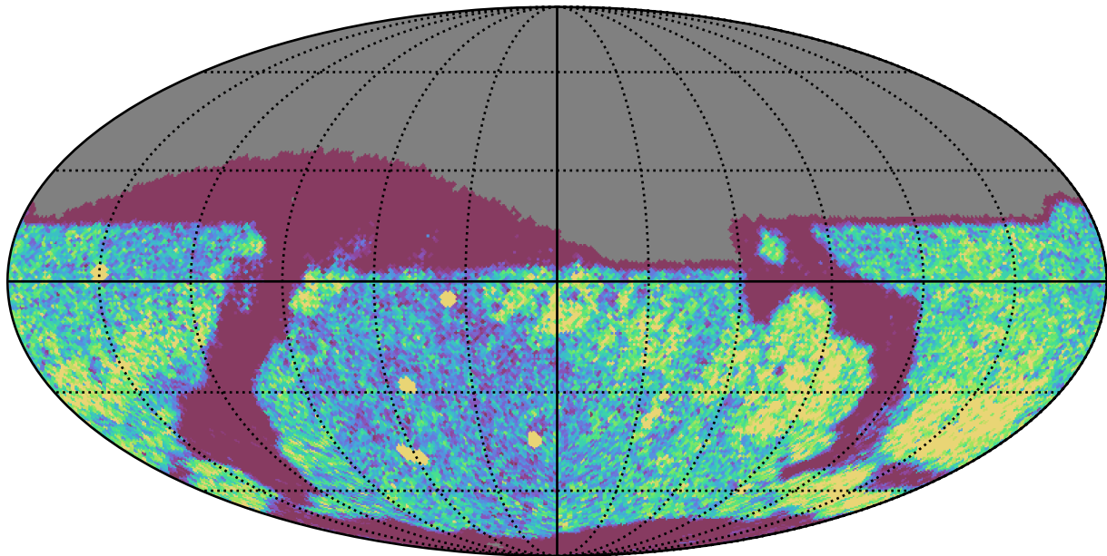
mw_roll_bulge_v3.3_10yrs Yr 1 r band: NVisits
