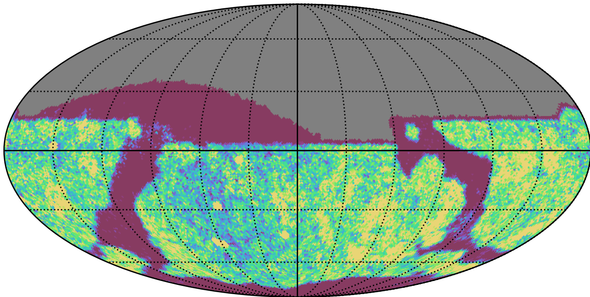
mw_roll_bulge_v3.3_10yrs Yr 1 i band: NVisits
