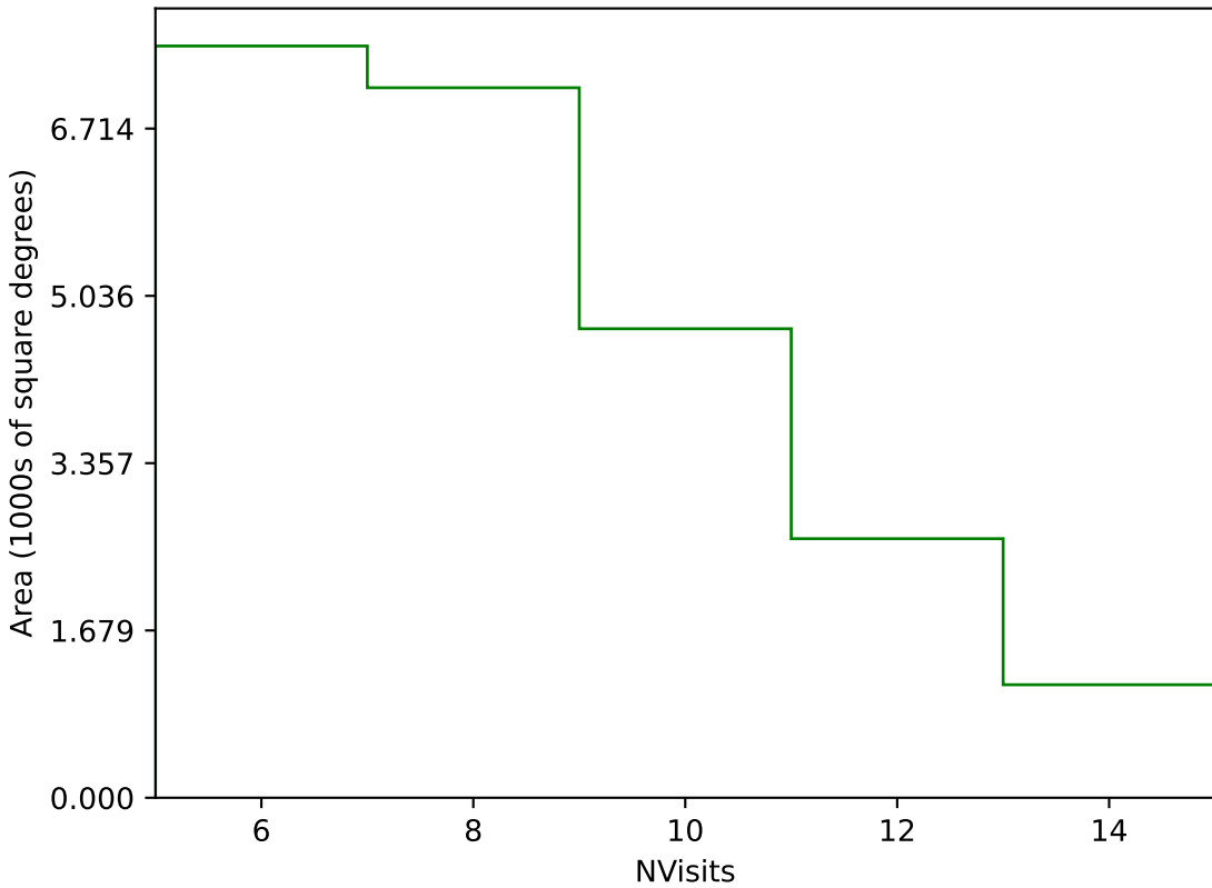
mw_roll_bulge_v3.3_10yrs Yr 1 g band: NVisits
