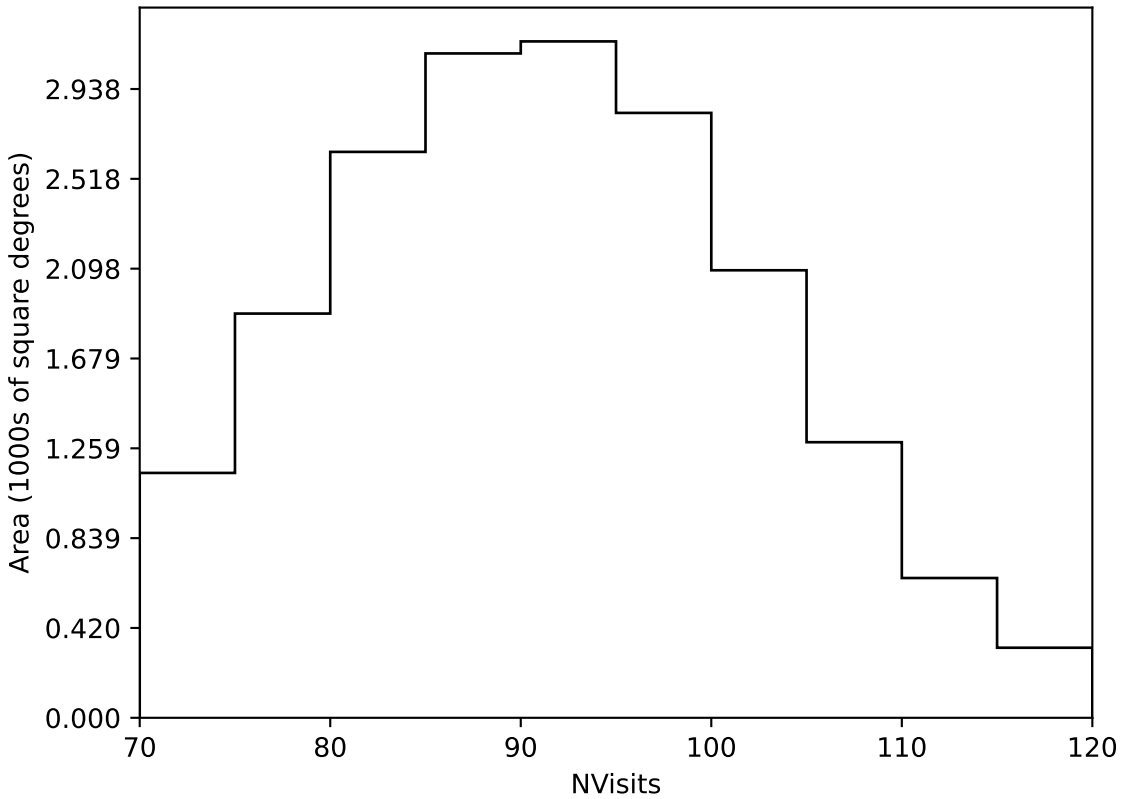
mw_roll_bulge_v3.3_10yrs Yr 1 all bands: NVisits
