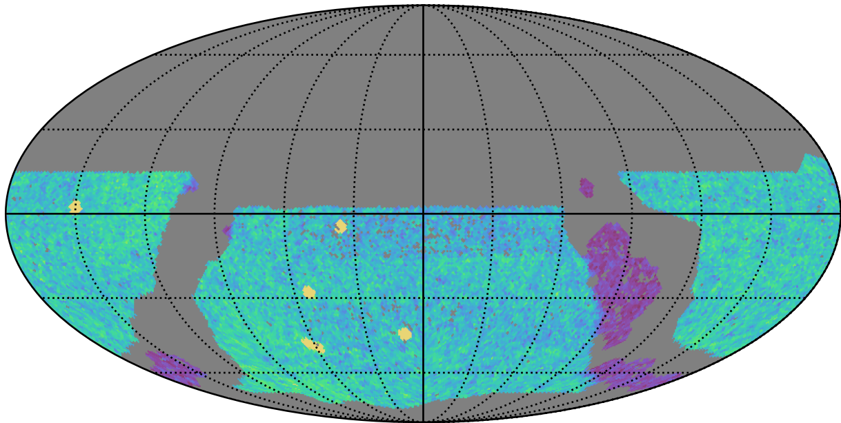
mw_roll_bulge_v3.3_10yrs WFD u band: NVisits
