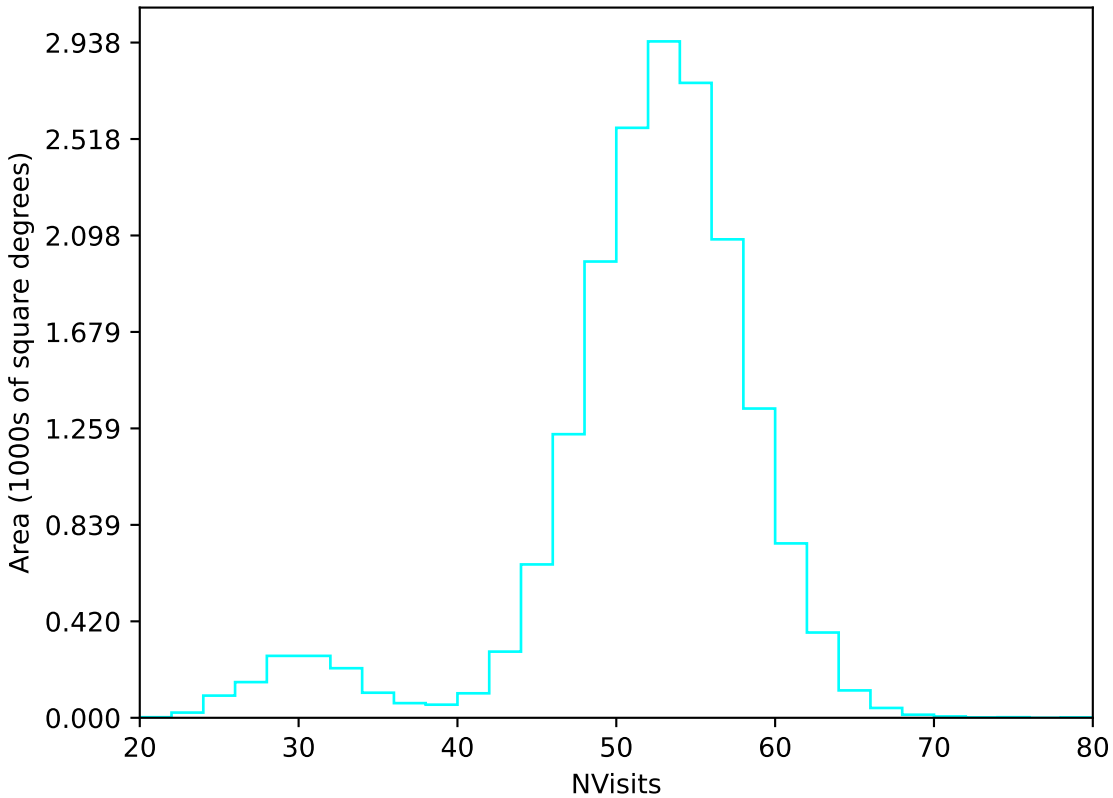
mw_roll_bulge_v3.3_10yrs WFD u band: NVisits
