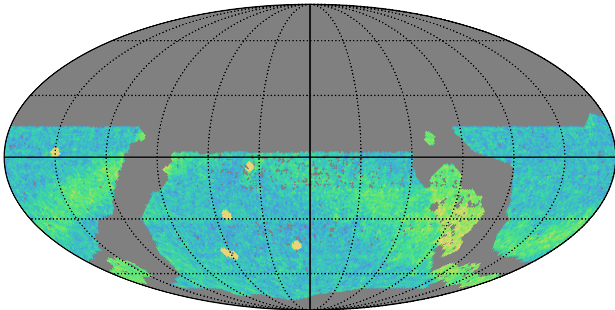
mw_roll_bulge_v3.3_10yrs WFD r band: NVisits
