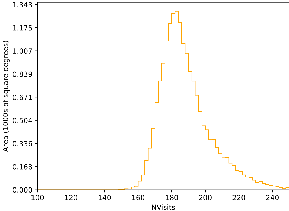
mw_roll_bulge_v3.3_10yrs WFD r band: NVisits
