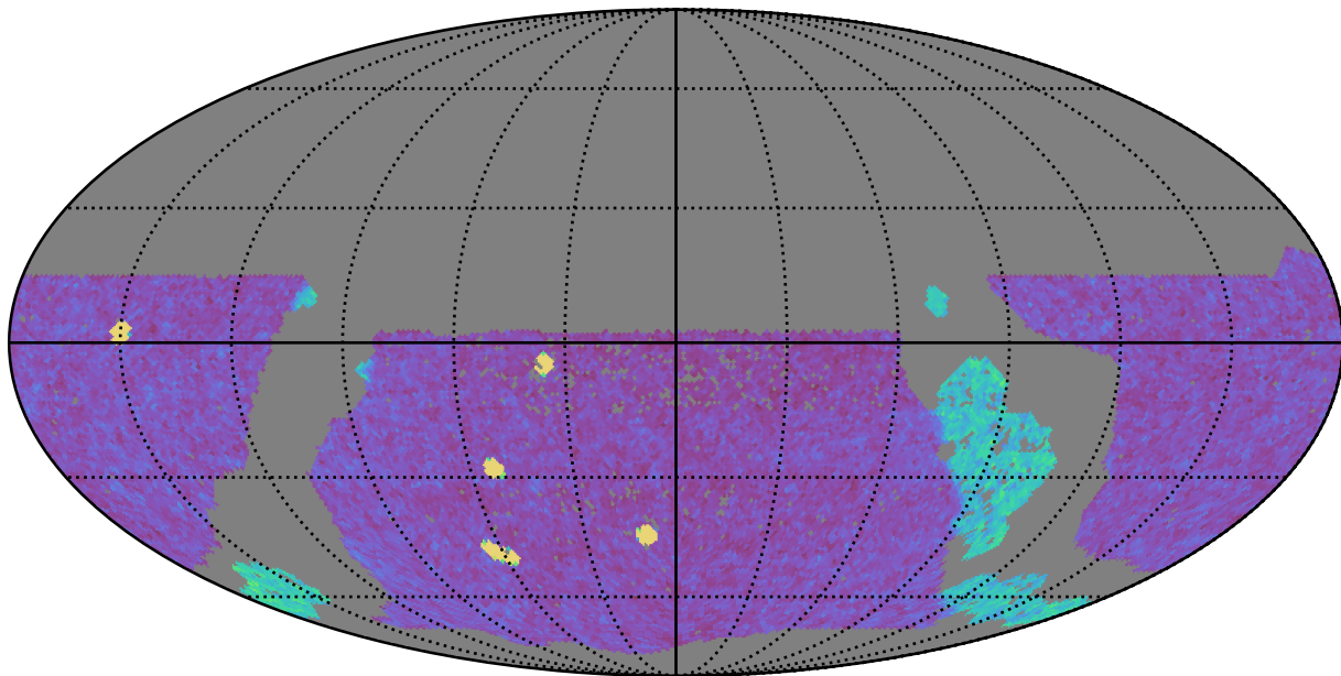
mw_roll_bulge_v3.3_10yrs WFD g band: NVisits
