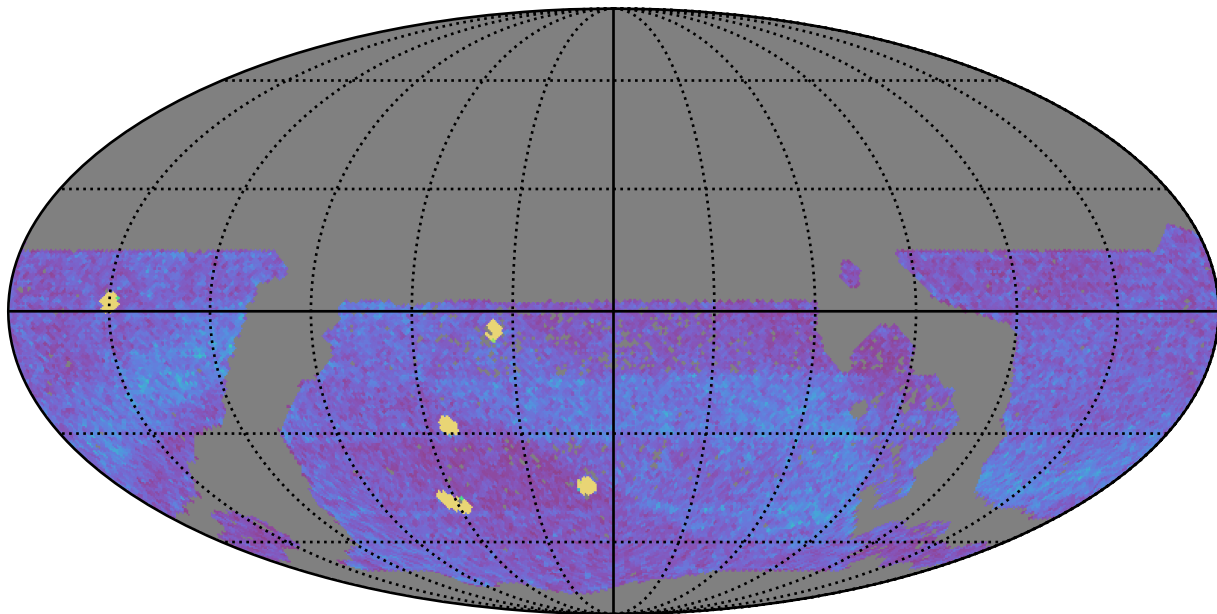
mw_roll_bulge_v3.3_10yrs WFD all bands: NVisits
