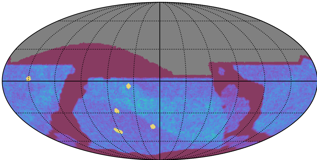
mw_roll_bulge_v3.3_10yrs All sky z band: NVisits
