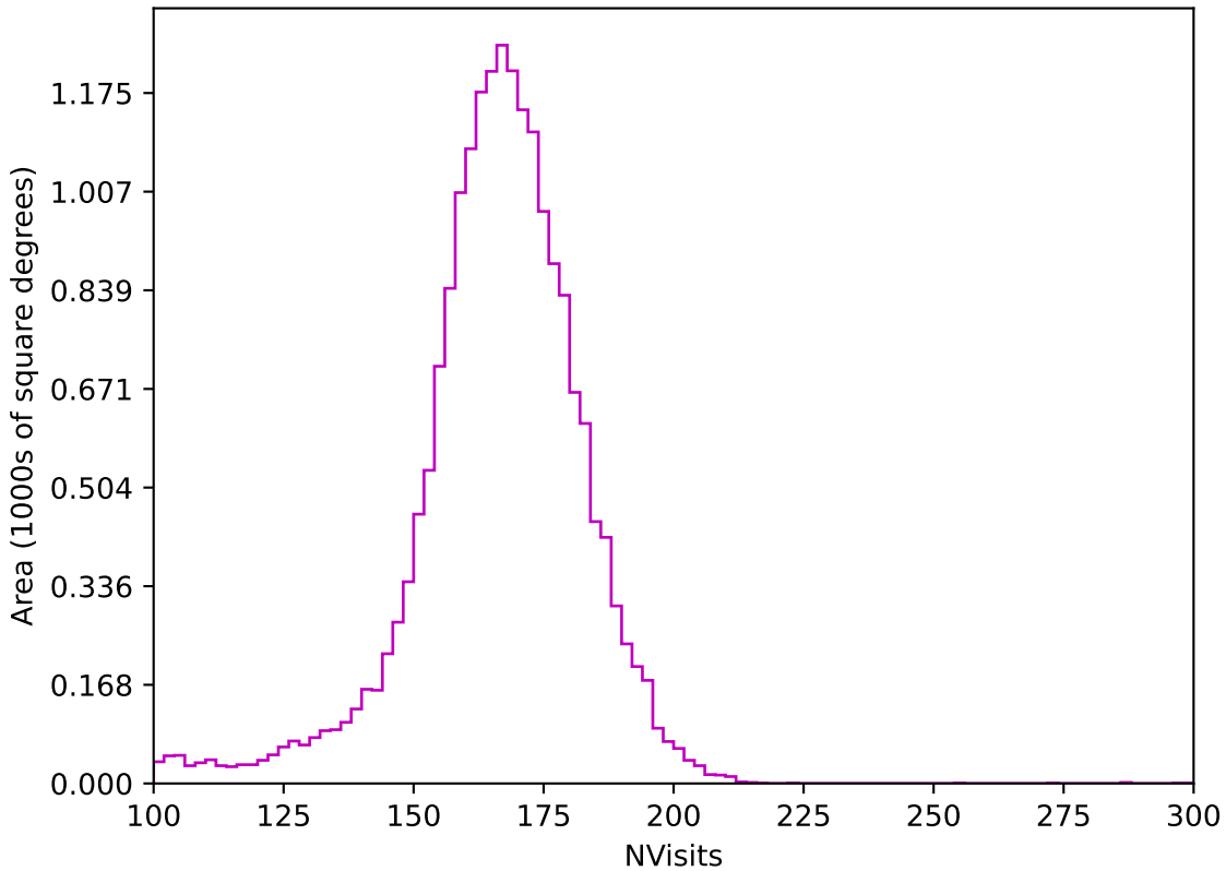
mw_roll_bulge_v3.3_10yrs All sky z band: NVisits
