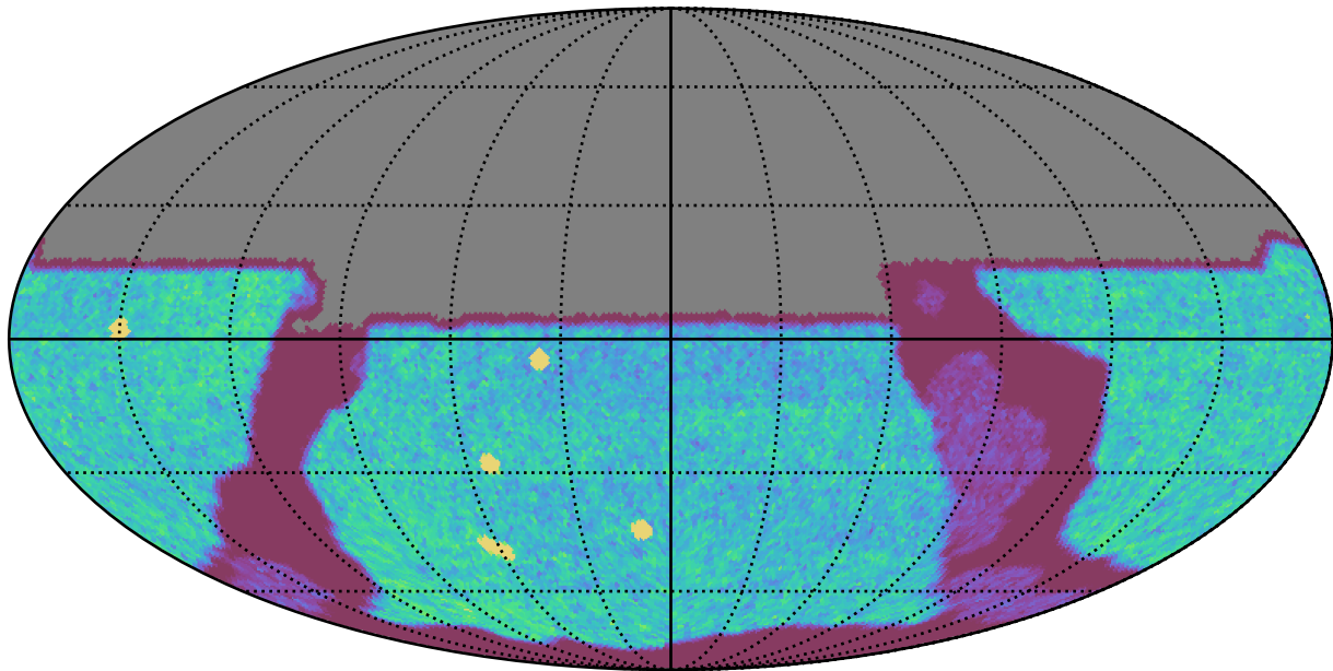
mw_roll_bulge_v3.3_10yrs All sky u band: NVisits
