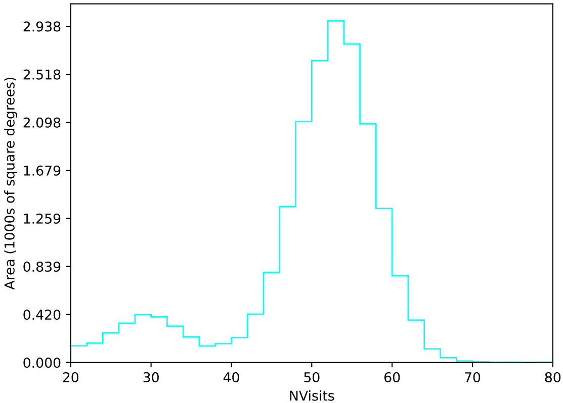
mw_roll_bulge_v3.3_10yrs All sky u band: NVisits
