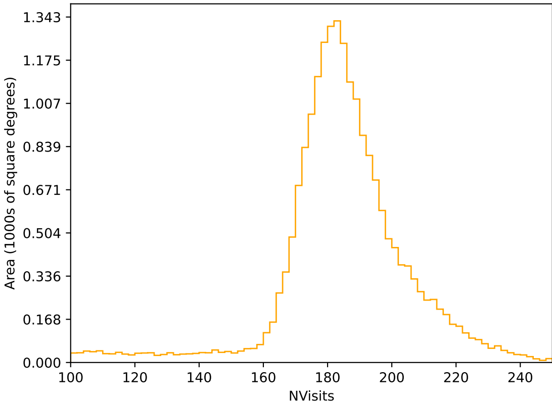
mw_roll_bulge_v3.3_10yrs All sky r band: NVisits
