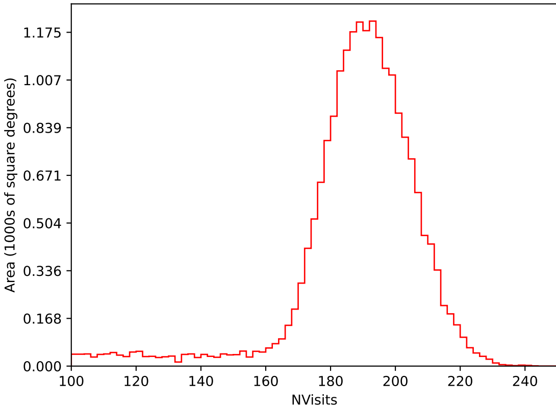
mw_roll_bulge_v3.3_10yrs All sky i band: NVisits
