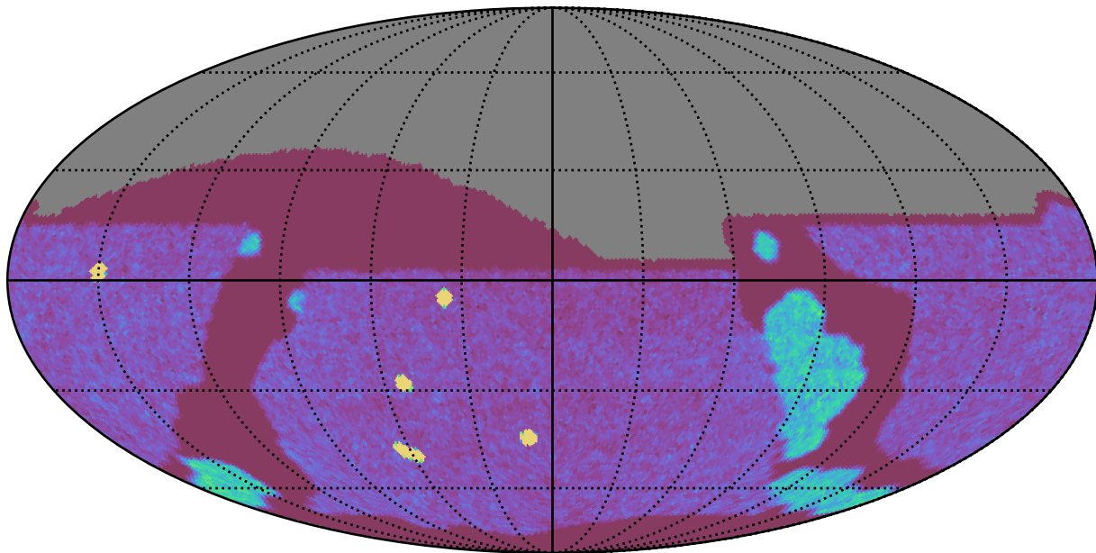
mw_roll_bulge_v3.3_10yrs All sky g band: NVisits
