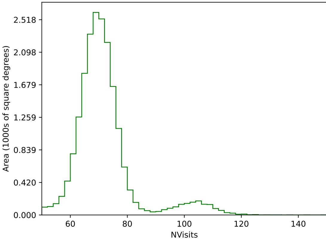
mw_roll_bulge_v3.3_10yrs All sky g band: NVisits
