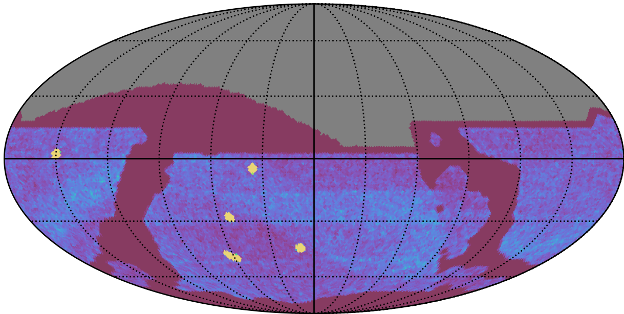
mw_roll_bulge_v3.3_10yrs All sky all bands: NVisits
