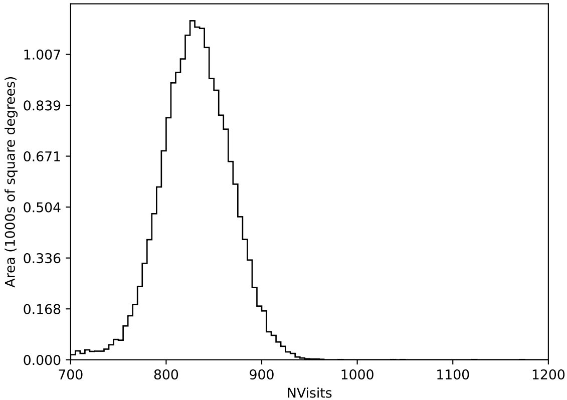
mw_roll_bulge_v3.3_10yrs All sky all bands: NVisits
