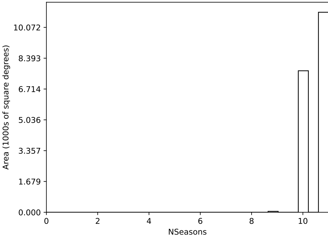
mw_roll_bulge_v3.3_10yrs WFD all bands: NSeasons
