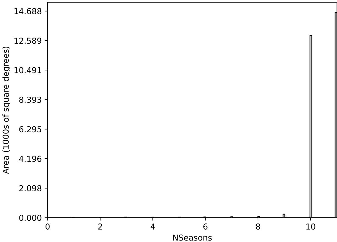
mw_roll_bulge_v3.3_10yrs All sky all bands: NSeasons
