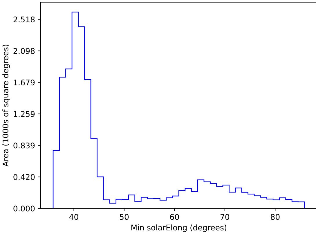
mw_roll_bulge_v3.3_10yrs WFD z band: Min solarElong
