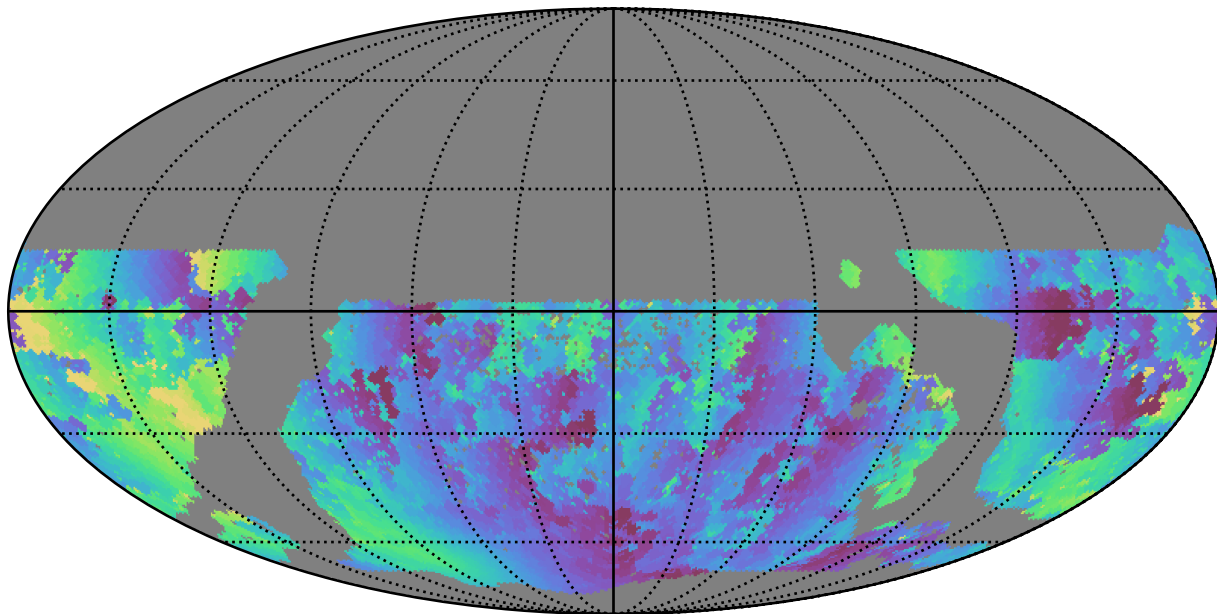
mw_roll_bulge_v3.3_10yrs WFD u band: Min solarElong
