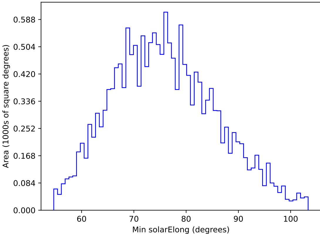
mw_roll_bulge_v3.3_10yrs WFD u band: Min solarElong
