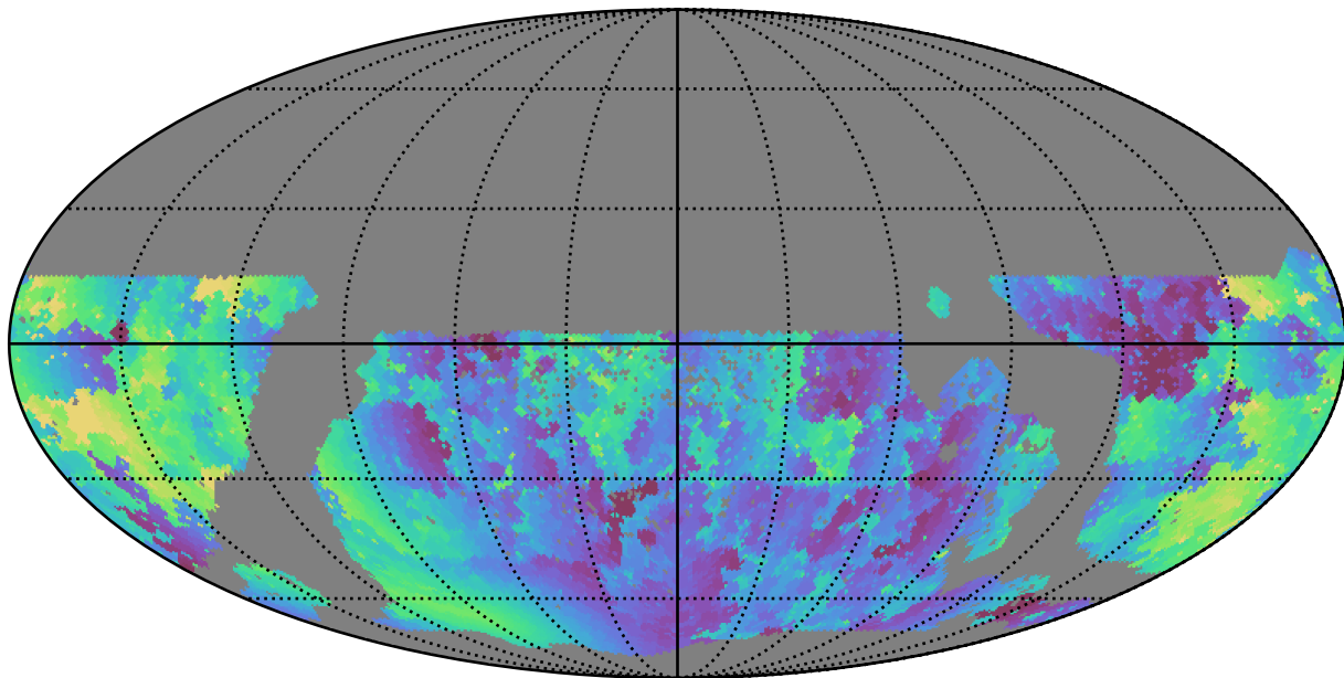
mw_roll_bulge_v3.3_10yrs WFD g band: Min solarElong
