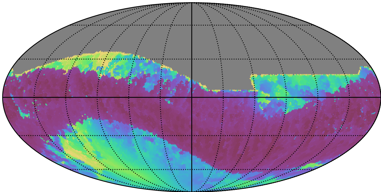
mw_roll_bulge_v3.3_10yrs All sky z band: Min solarElong
